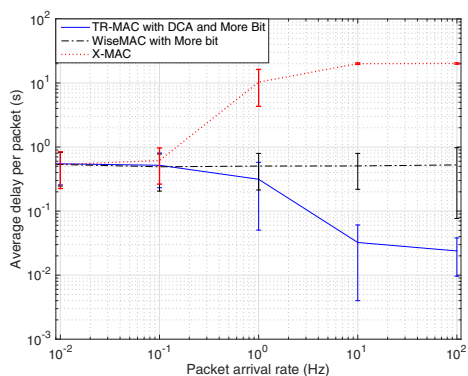
Fig. 4: Average delay per packet with varying traffic
