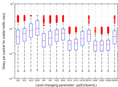
Fig. 7: Delay per packet for stable traffic
